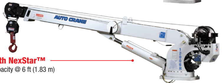
10006H Series with NexStar™ 10,000 lb (4,536 kg) capacity @ 6 ft (1.83 m)
